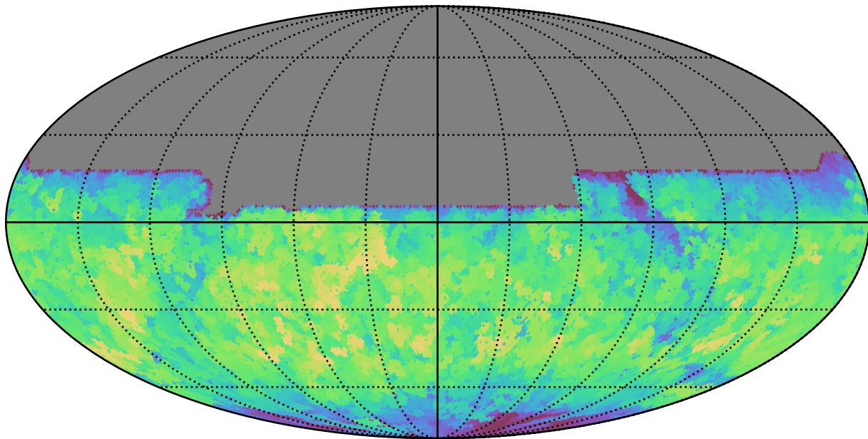
ddf_half_v3.4_10yrs All sky y band: Max saturation_mag
