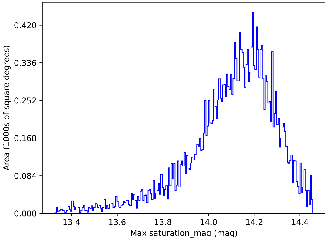
ddf_half_v3.4_10yrs All sky y band: Max saturation_mag
