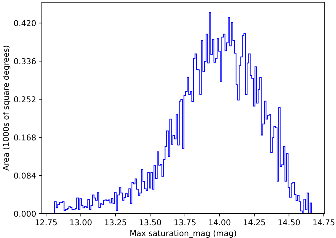
ddf_half_v3.4_10yrs All sky u band: Max saturation_mag
