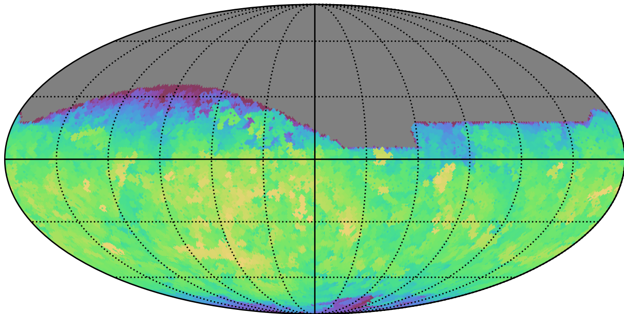
ddf_half_v3.4_10yrs All sky r band: Max saturation_mag
