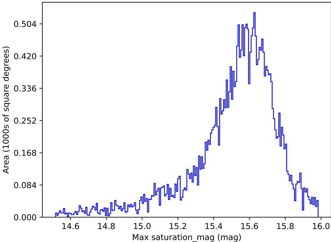
ddf_half_v3.4_10yrs All sky i band: Max saturation_mag
