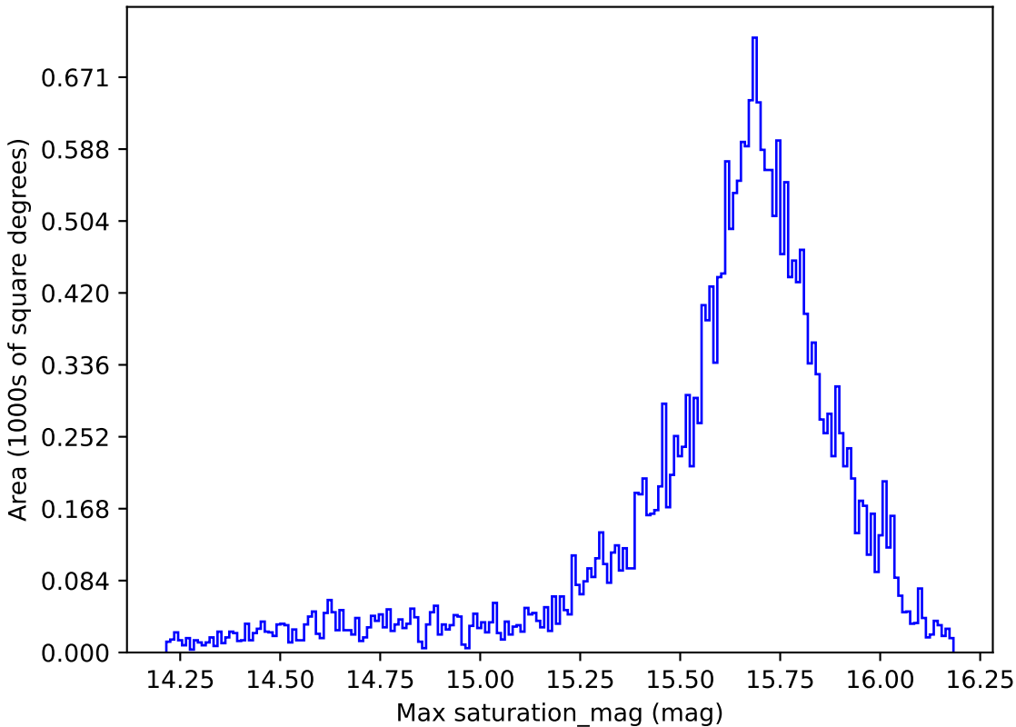
ddf_half_v3.4_10yrs All sky g band: Max saturation_mag
