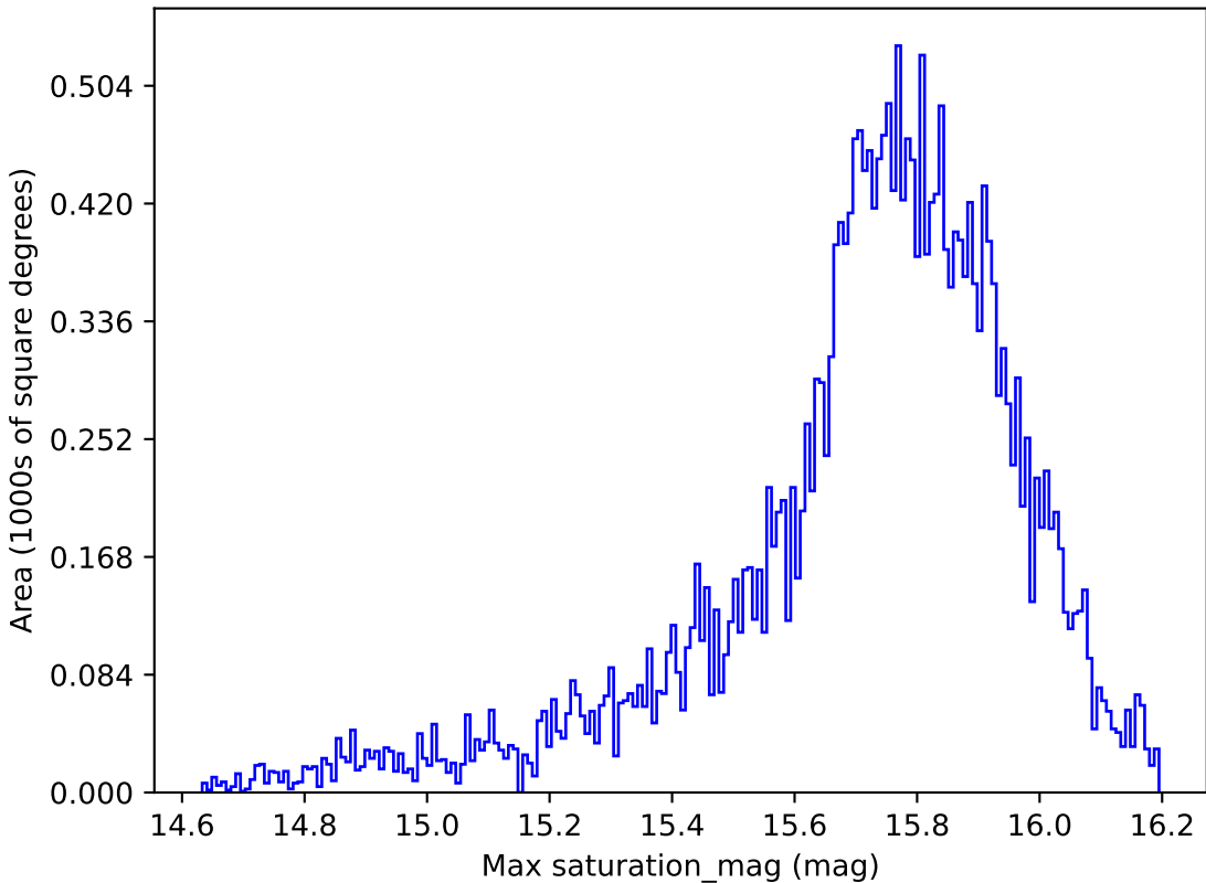
ddf_half_v3.4_10yrs All sky all bands: Max saturation_mag
