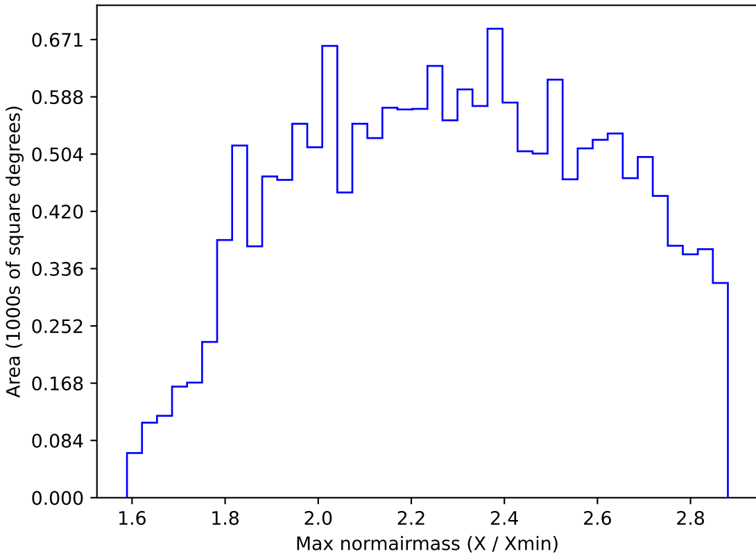
ddf_half_v3.4_10yrs WFD z band: Max normairmass
