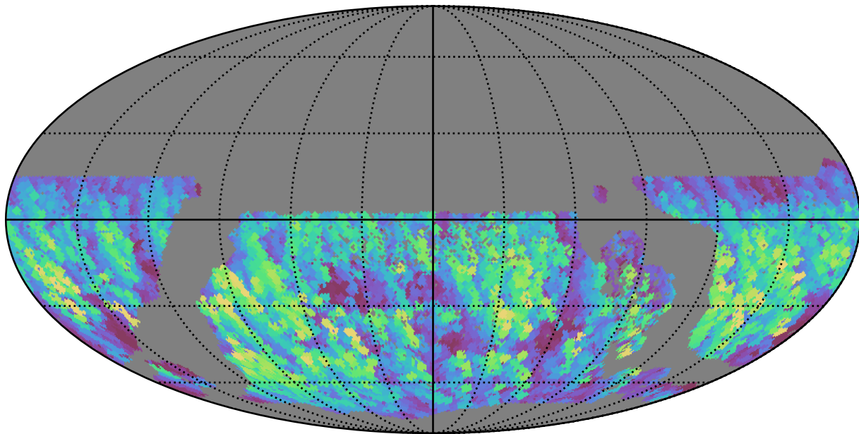
ddf_half_v3.4_10yrs WFD y band: Max normairmass
