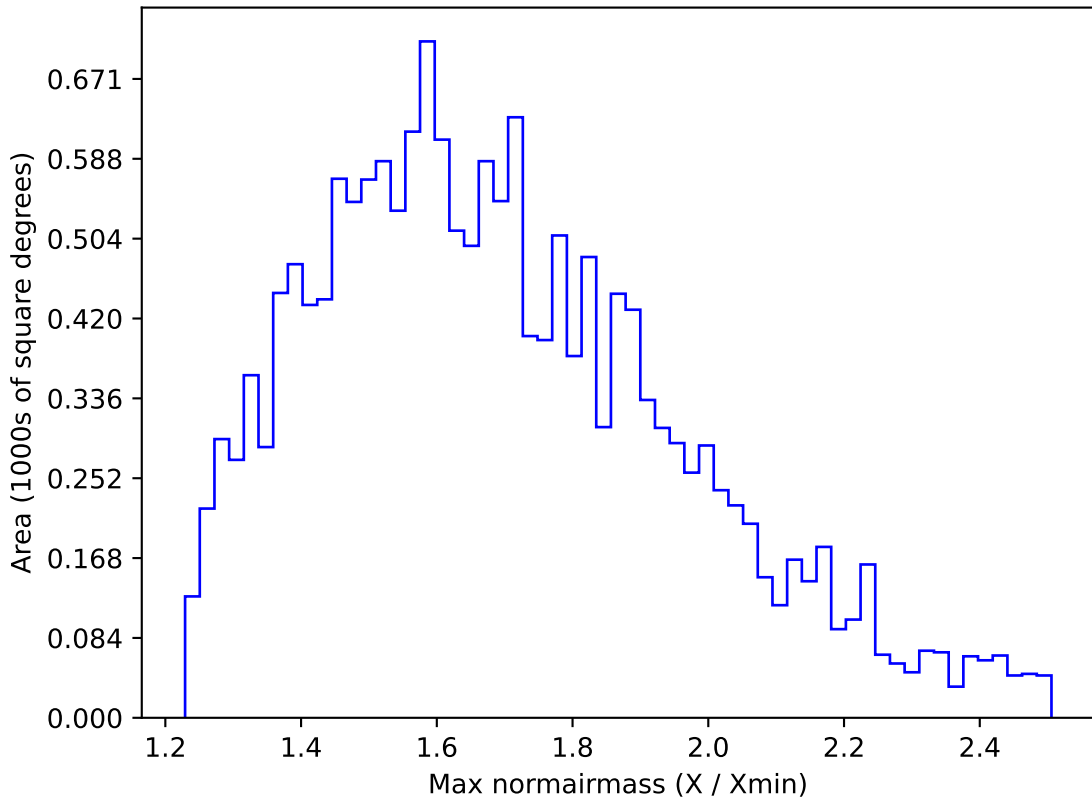
ddf_half_v3.4_10yrs WFD u band: Max normairmass
