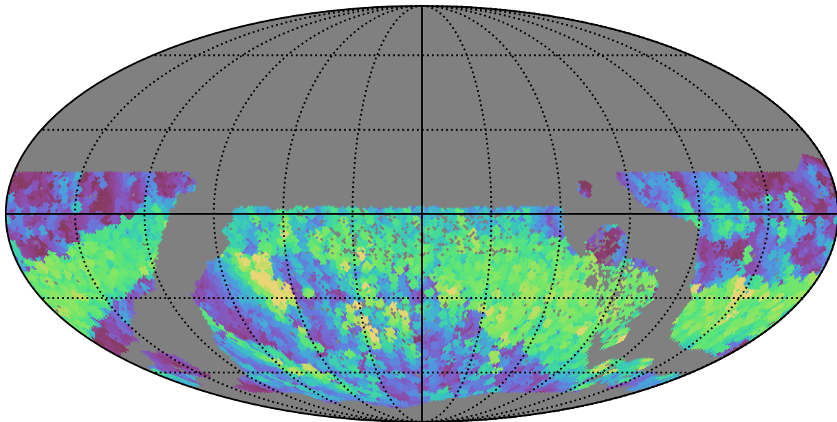
ddf_half_v3.4_10yrs WFD r band: Max normairmass
