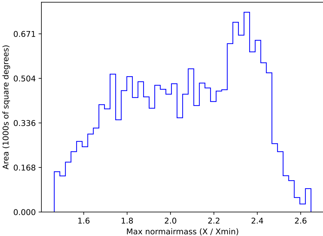
ddf_half_v3.4_10yrs WFD r band: Max normairmass
