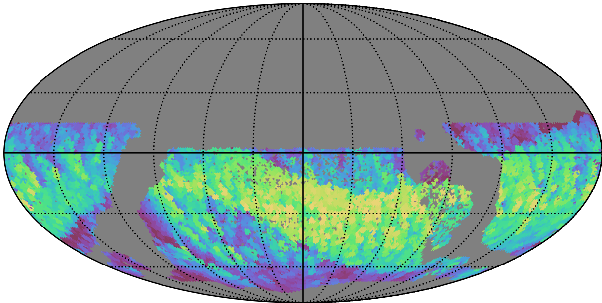
ddf_half_v3.4_10yrs WFD i band: Max normairmass
