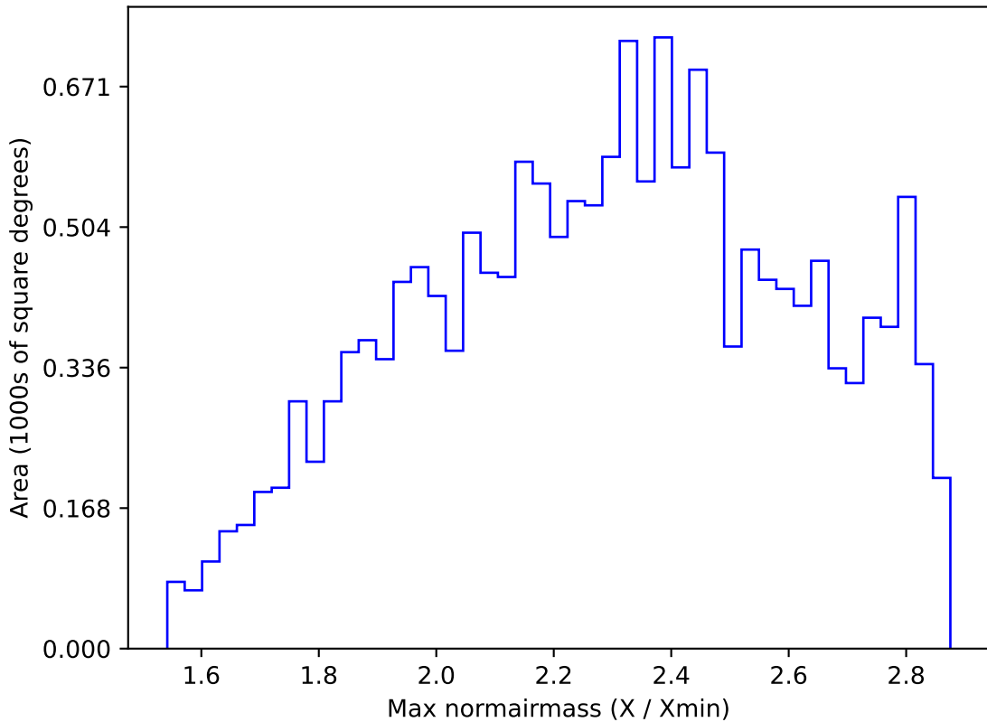
ddf_half_v3.4_10yrs WFD i band: Max normairmass
