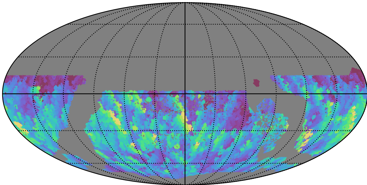
ddf_half_v3.4_10yrs WFD g band: Max normairmass
