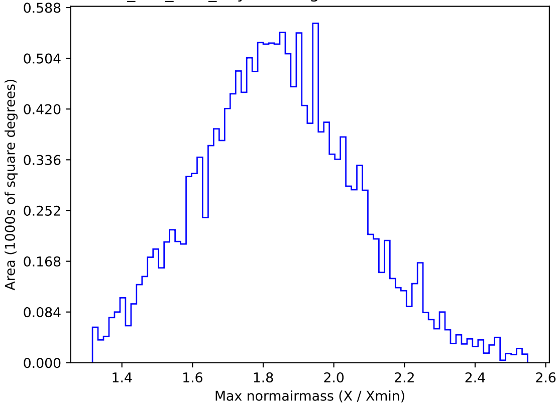
ddf_half_v3.4_10yrs WFD g band: Max normairmass
