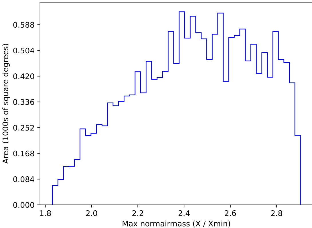
ddf_half_v3.4_10yrs WFD all bands: Max normairmass
