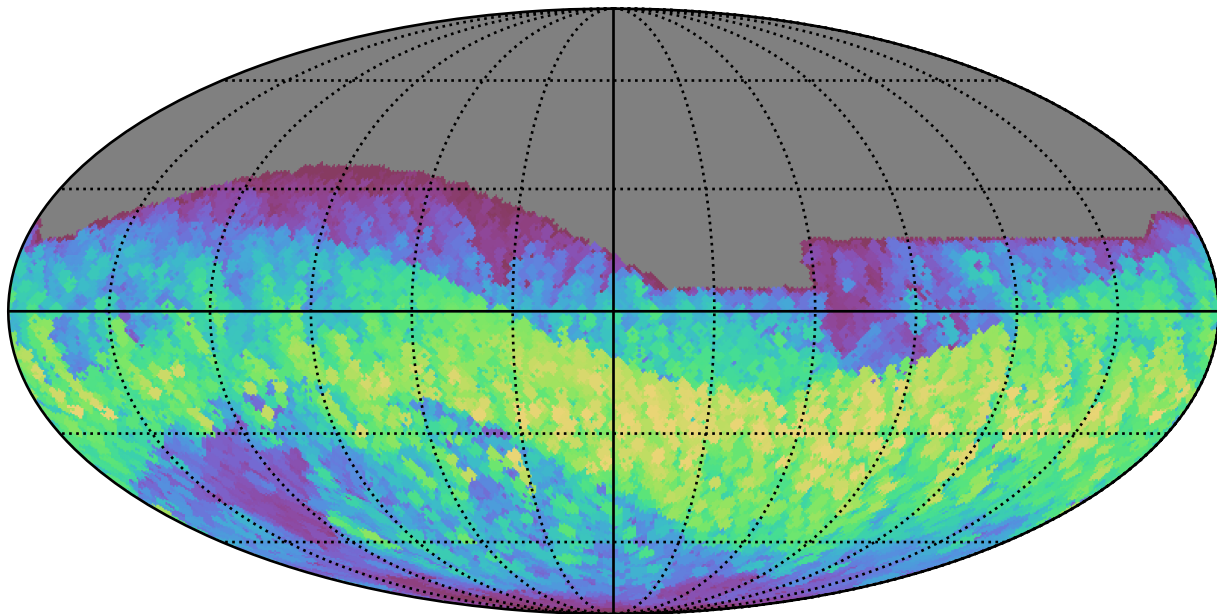
ddf_half_v3.4_10yrs All sky z band: Max normairmass
