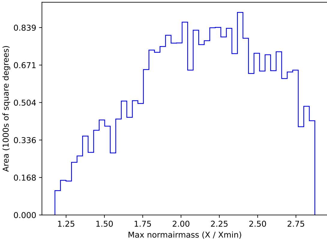
ddf_half_v3.4_10yrs All sky z band: Max normairmass
