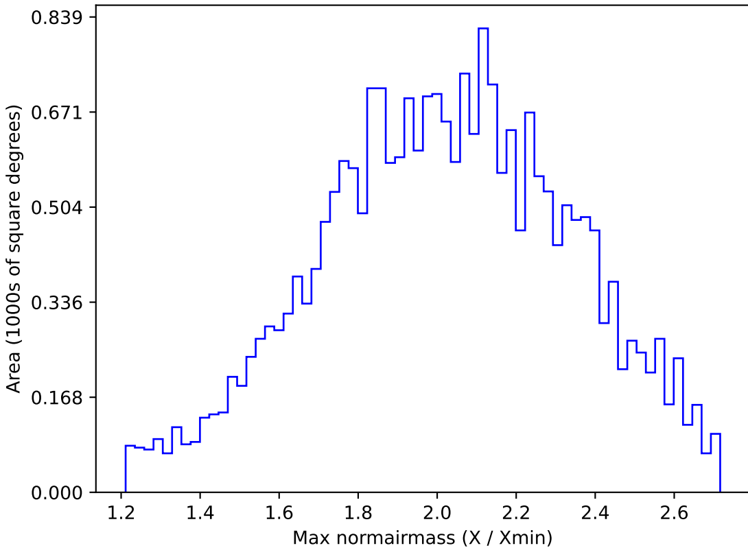
ddf_half_v3.4_10yrs All sky y band: Max normairmass
