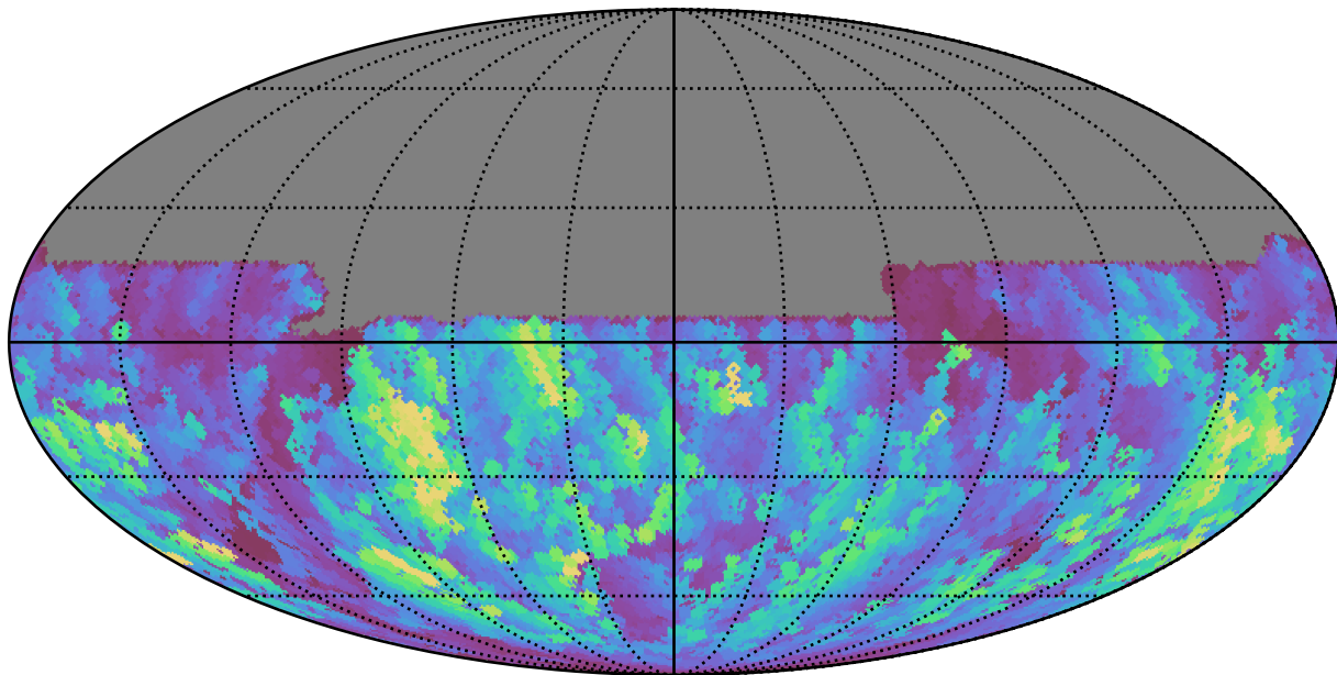
ddf_half_v3.4_10yrs All sky u band: Max normairmass
