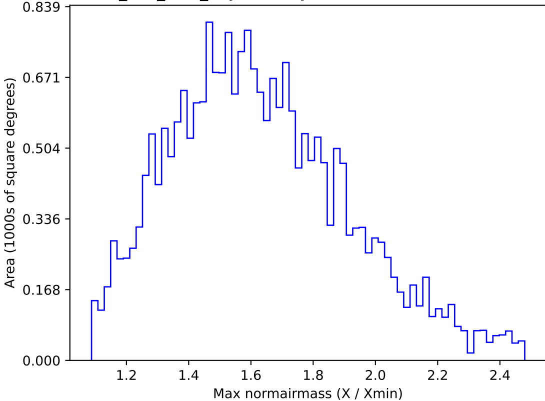
ddf_half_v3.4_10yrs All sky u band: Max normairmass
