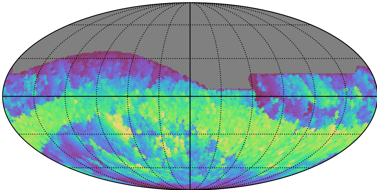
ddf_half_v3.4_10yrs All sky r band: Max normairmass
