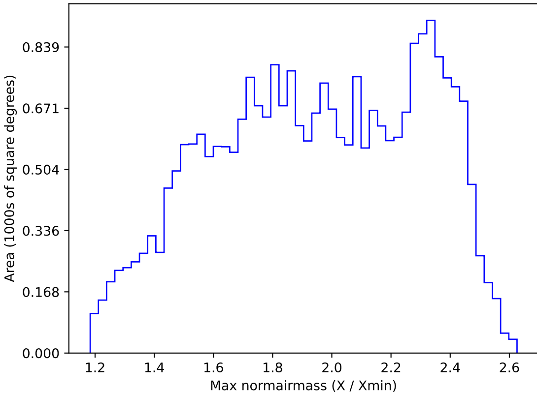
ddf_half_v3.4_10yrs All sky r band: Max normairmass
