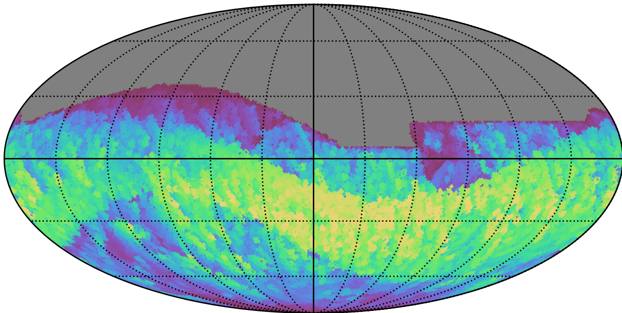
ddf_half_v3.4_10yrs All sky i band: Max normairmass
