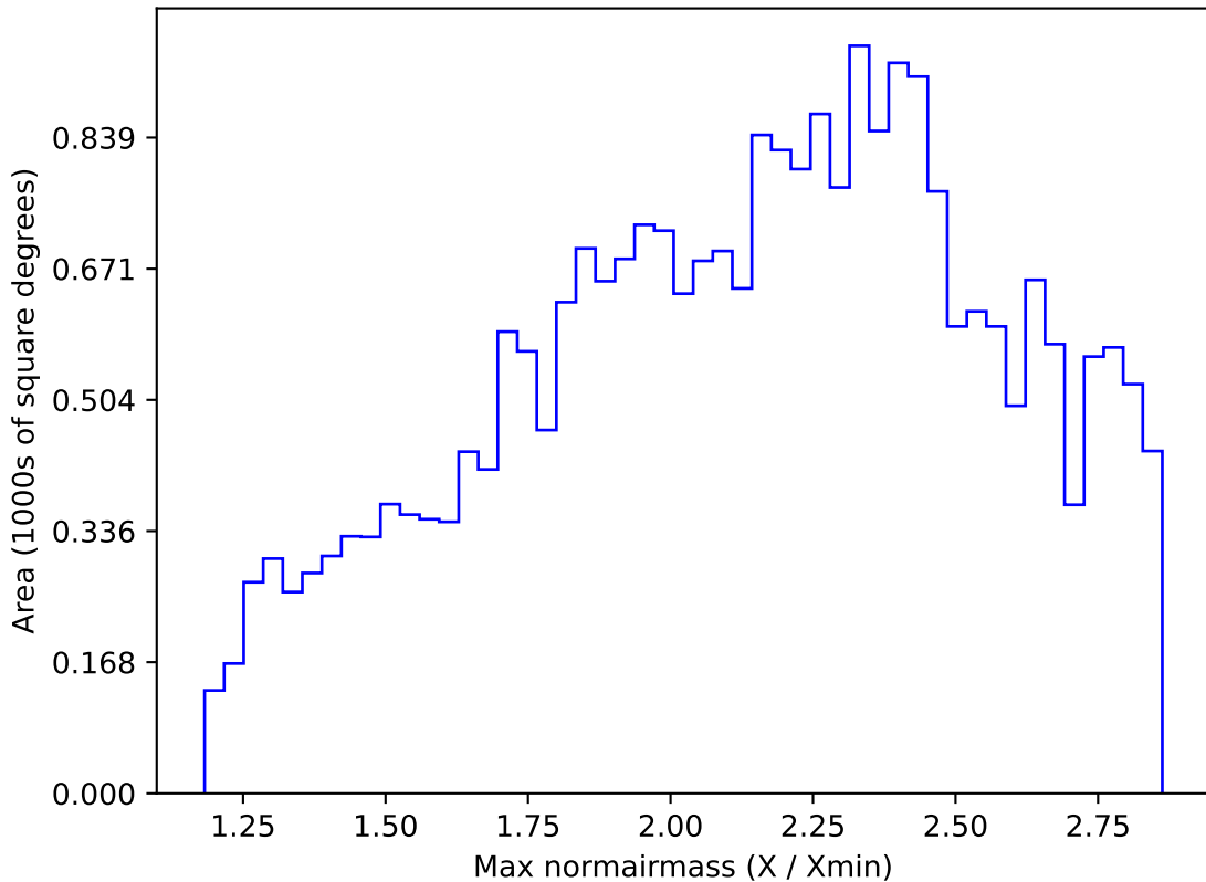
ddf_half_v3.4_10yrs All sky i band: Max normairmass
