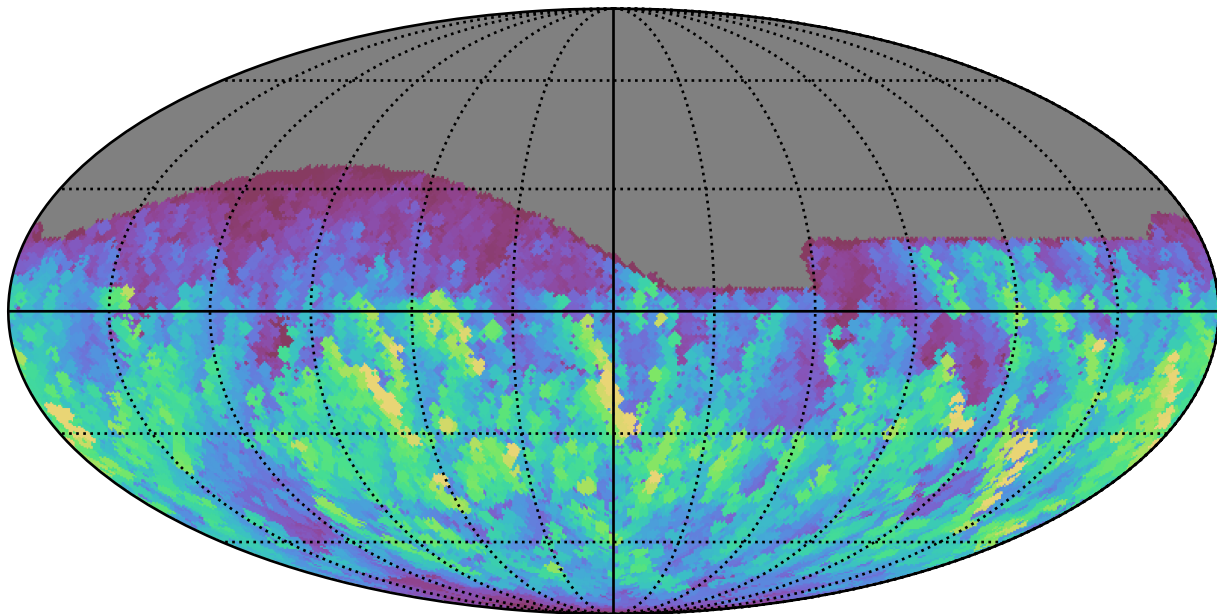
ddf_half_v3.4_10yrs All sky g band: Max normairmass
