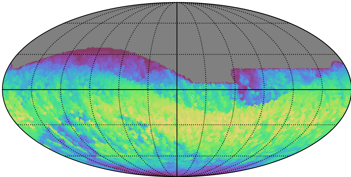
ddf_half_v3.4_10yrs All sky all bands: Max normairmass
