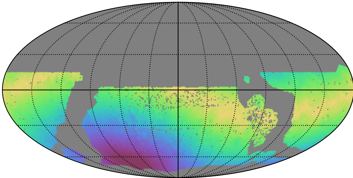
ddf_half_v3.4_10yrs WFD z band: Max moonDistance
