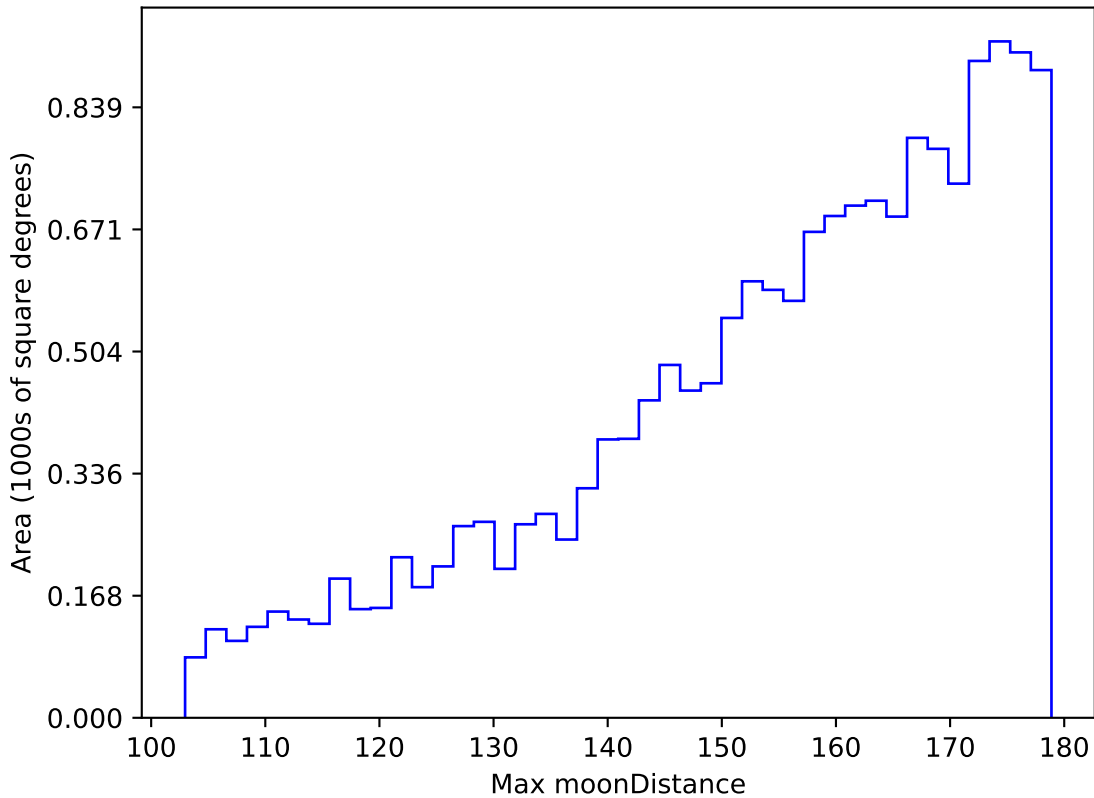
ddf_half_v3.4_10yrs WFD z band: Max moonDistance
