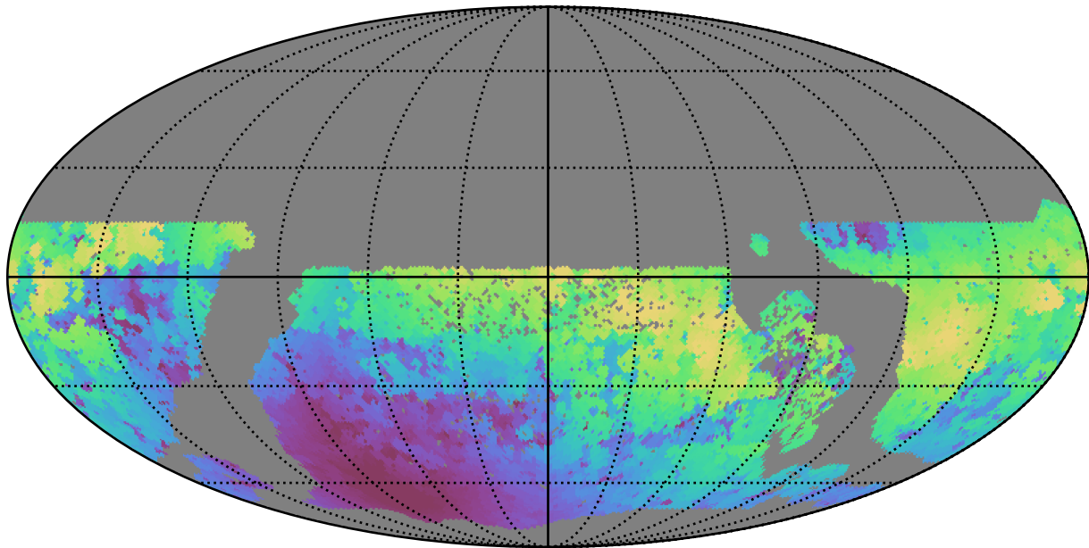
ddf_half_v3.4_10yrs WFD y band: Max moonDistance
