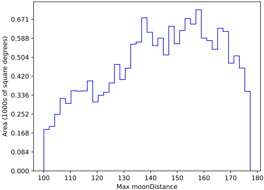
ddf_half_v3.4_10yrs WFD y band: Max moonDistance
