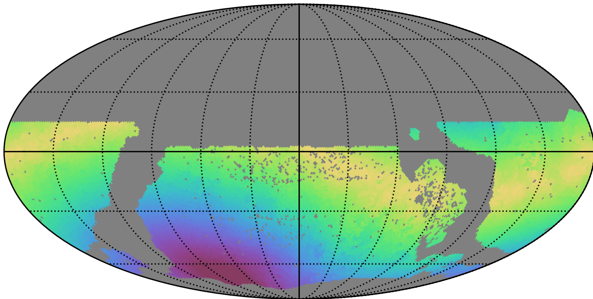
ddf_half_v3.4_10yrs WFD u band: Max moonDistance
