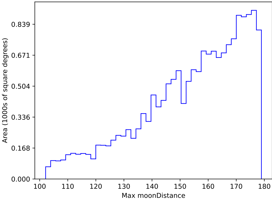
ddf_half_v3.4_10yrs WFD u band: Max moonDistance
