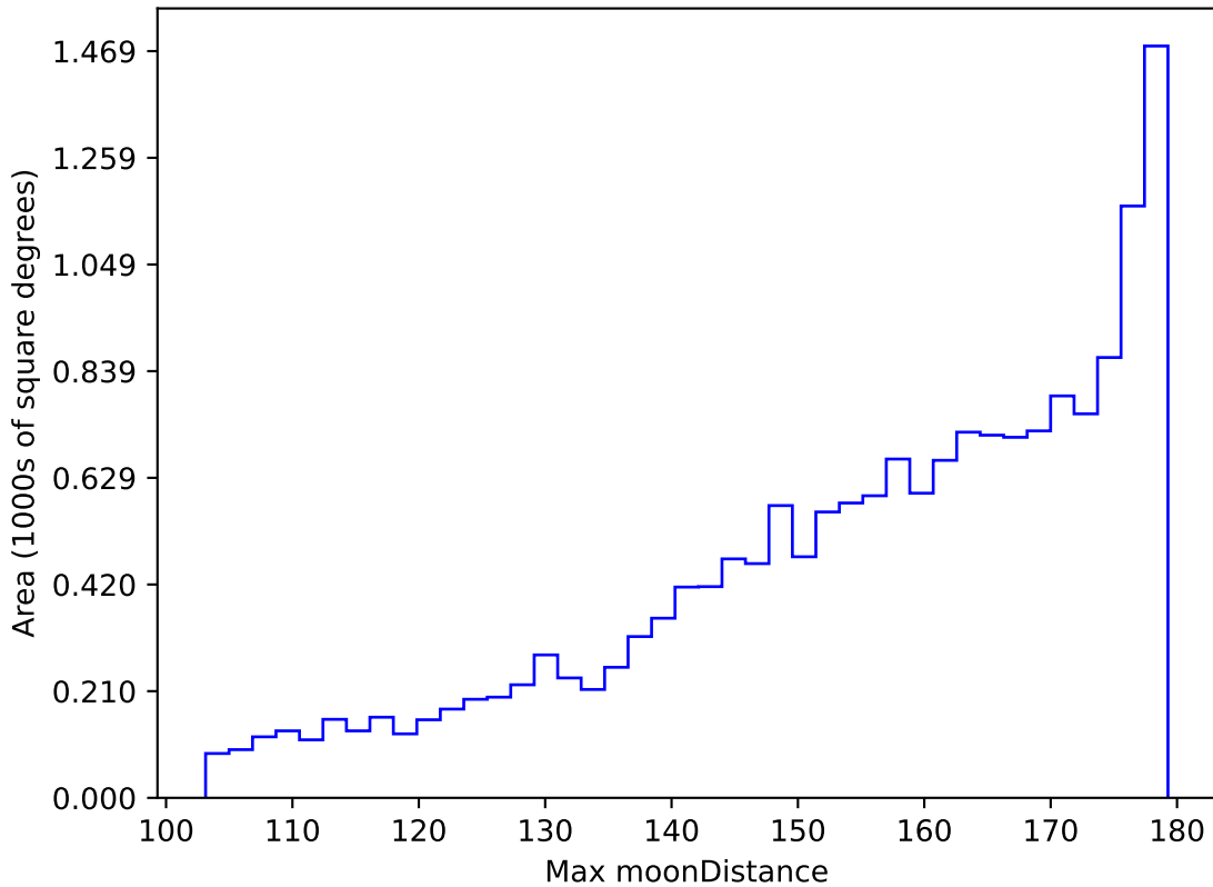
ddf_half_v3.4_10yrs WFD r band: Max moonDistance
