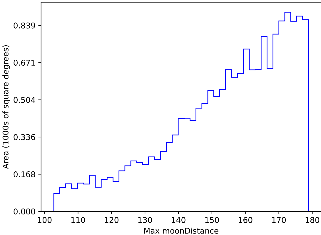
ddf_half_v3.4_10yrs WFD g band: Max moonDistance
