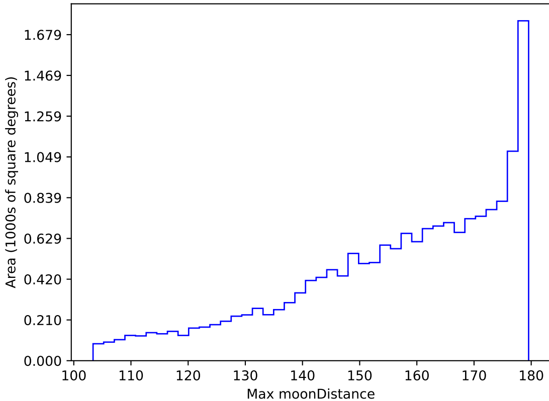
ddf_half_v3.4_10yrs WFD all bands: Max moonDistance
