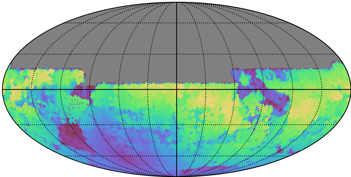
ddf_half_v3.4_10yrs All sky y band: Max moonDistance
