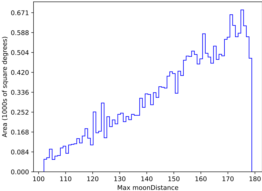
ddf_half_v3.4_10yrs All sky u band: Max moonDistance
