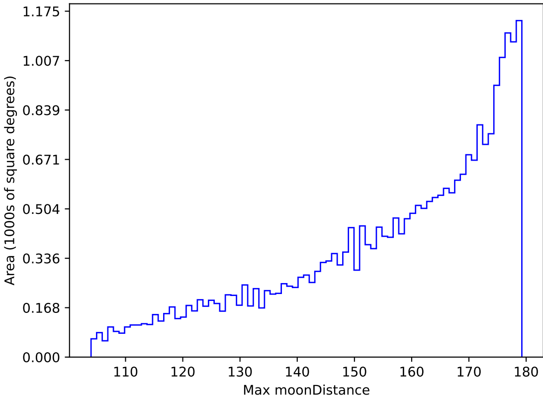
ddf_half_v3.4_10yrs All sky r band: Max moonDistance
