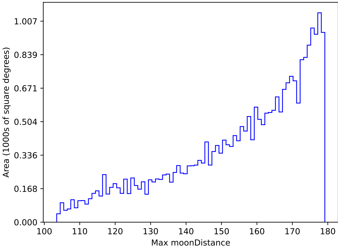
ddf_half_v3.4_10yrs All sky i band: Max moonDistance
