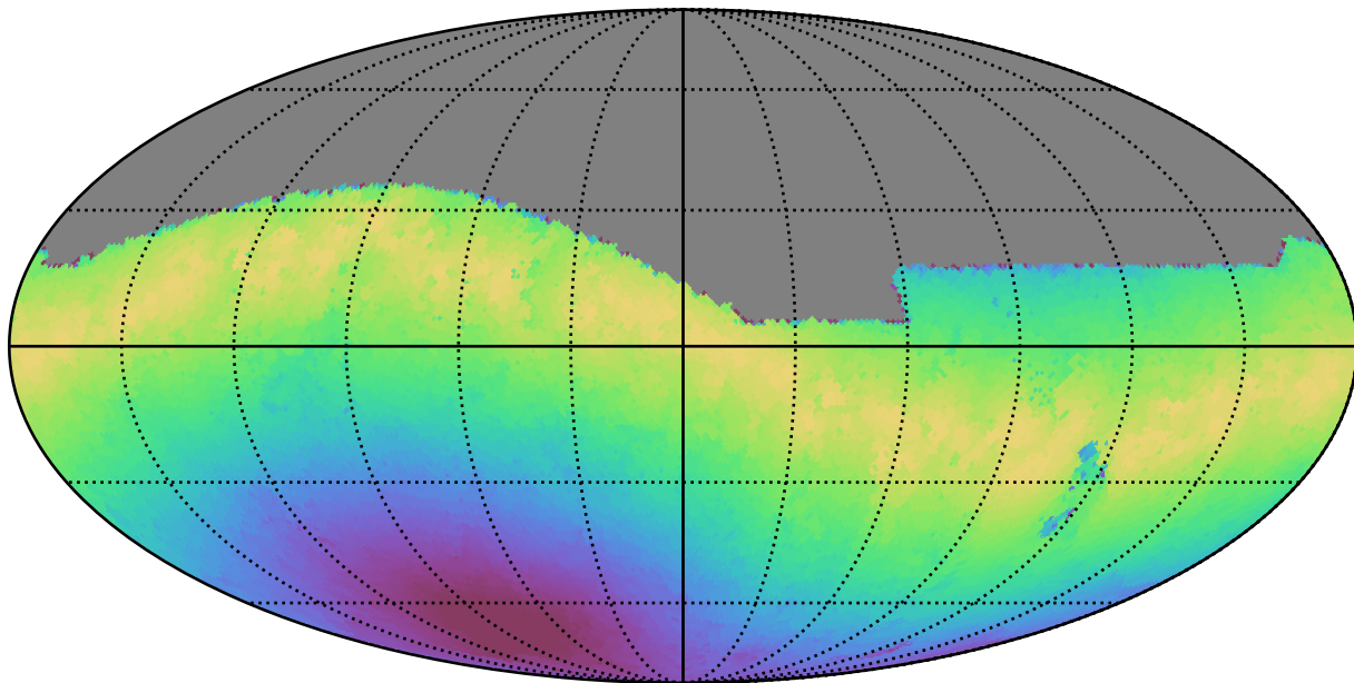
ddf_half_v3.4_10yrs All sky g band: Max moonDistance
