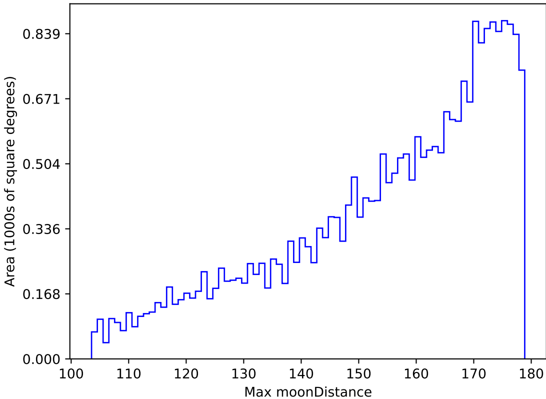
ddf_half_v3.4_10yrs All sky g band: Max moonDistance
