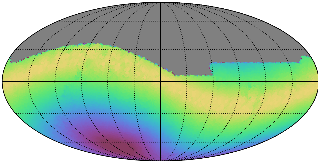
ddf_half_v3.4_10yrs All sky all bands: Max moonDistance
