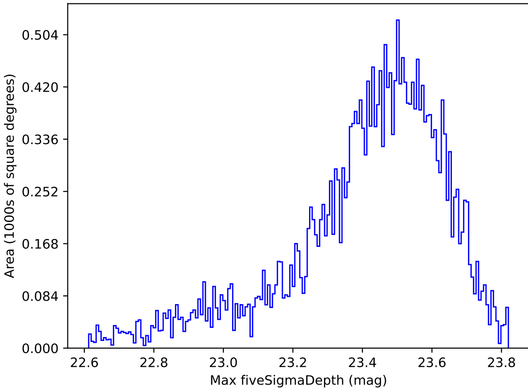
ddf_half_v3.4_10yrs Yr 1 z band: Max fiveSigmaDepth
