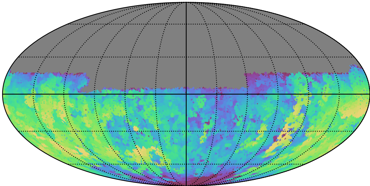
ddf_half_v3.4_10yrs Yr 1 u band: Max fiveSigmaDepth
