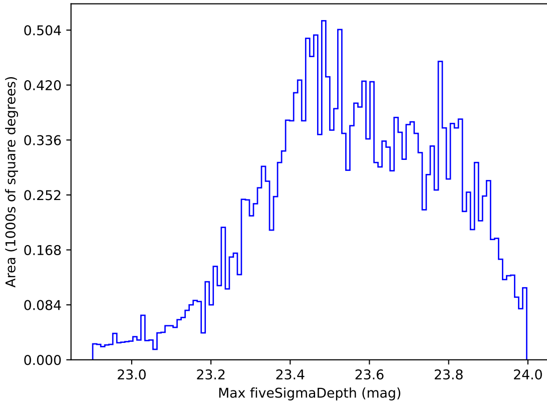
ddf_half_v3.4_10yrs Yr 1 u band: Max fiveSigmaDepth
