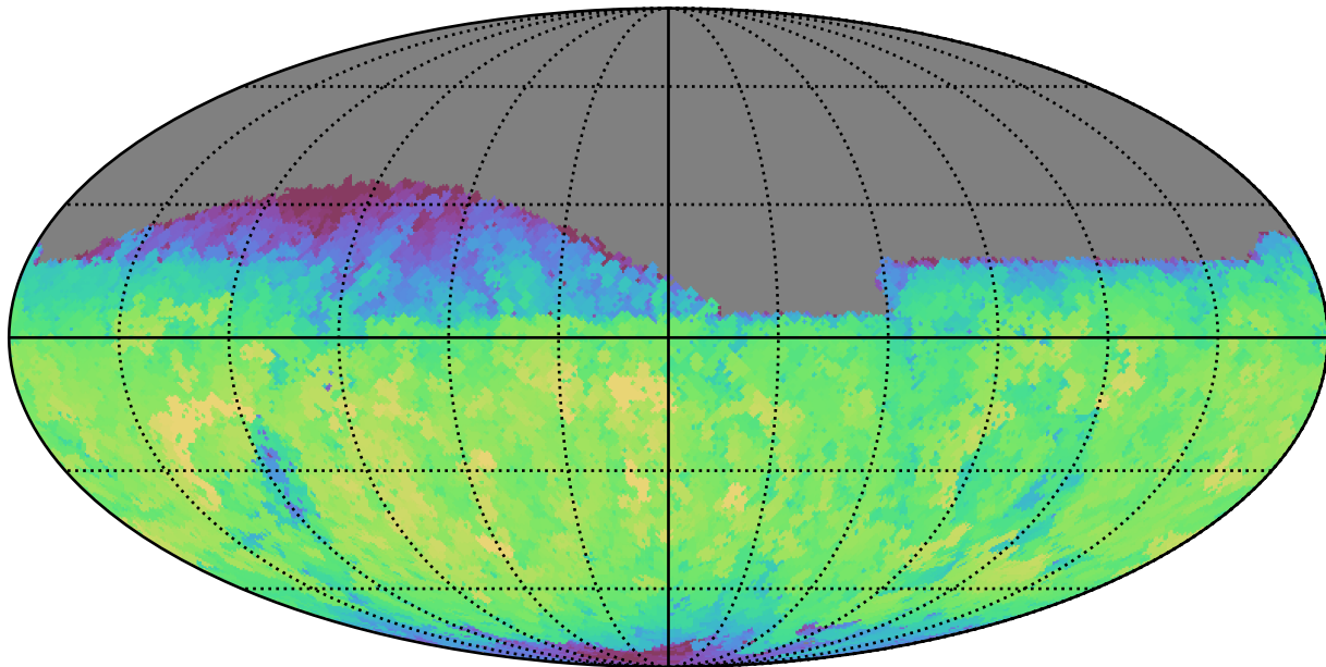
ddf_half_v3.4_10yrs Yr 1 i band: Max fiveSigmaDepth
