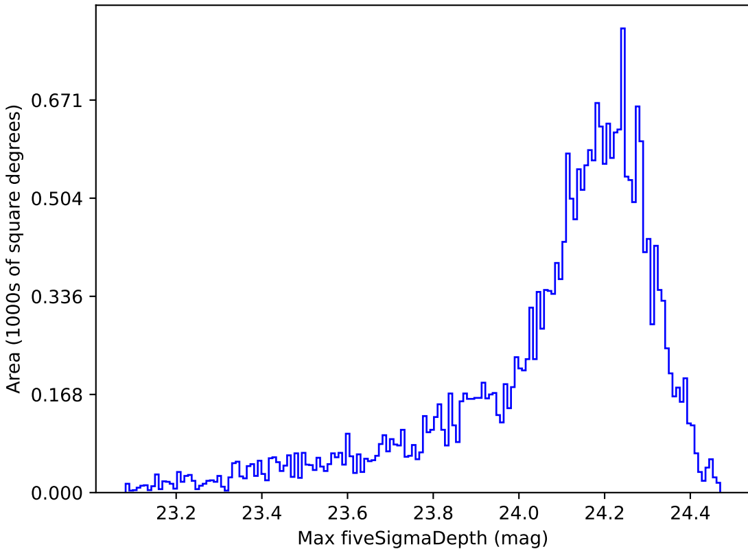
ddf_half_v3.4_10yrs Yr 1 i band: Max fiveSigmaDepth
