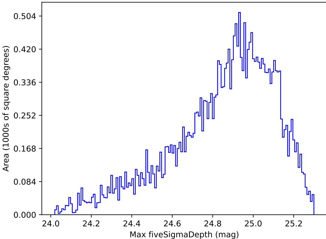
ddf_half_v3.4_10yrs Yr 1 g band: Max fiveSigmaDepth
